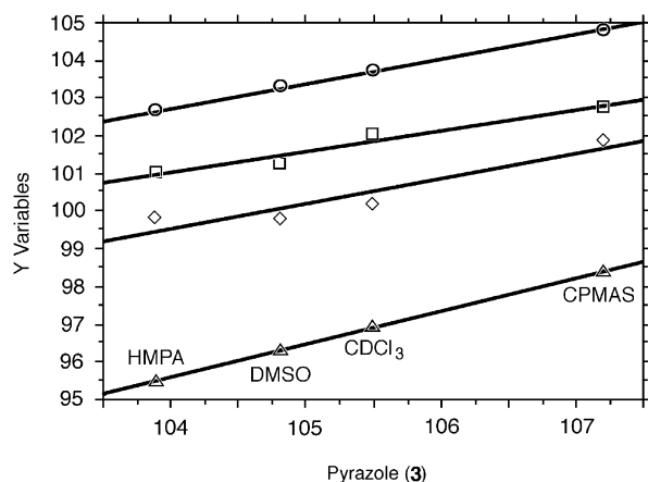
Fig. 2 ^{13}\text{C} chemical shifts of the C-4 of NH-pyrazoles: 3,5-dimethylpyrazole ( 4 , ○), 3(5)-methyl-5(3)-phenylpyrazole ( 17 , □), 3,5-di- tert -butylpyrazole ( 18 , △), 3,5-diphenylpyrazole ( 19 , ◇).
