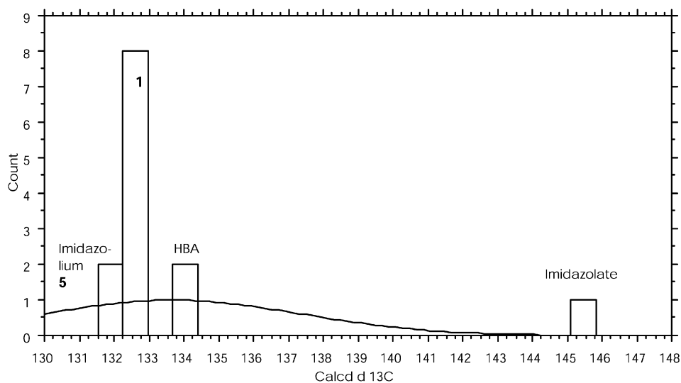
Fig. 3 ^{13}\text{C} chemical shifts of imidazole C-2.
